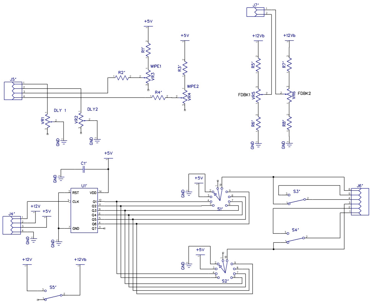
DISCRET11 V2.3 - Control board Syntonie 2018
