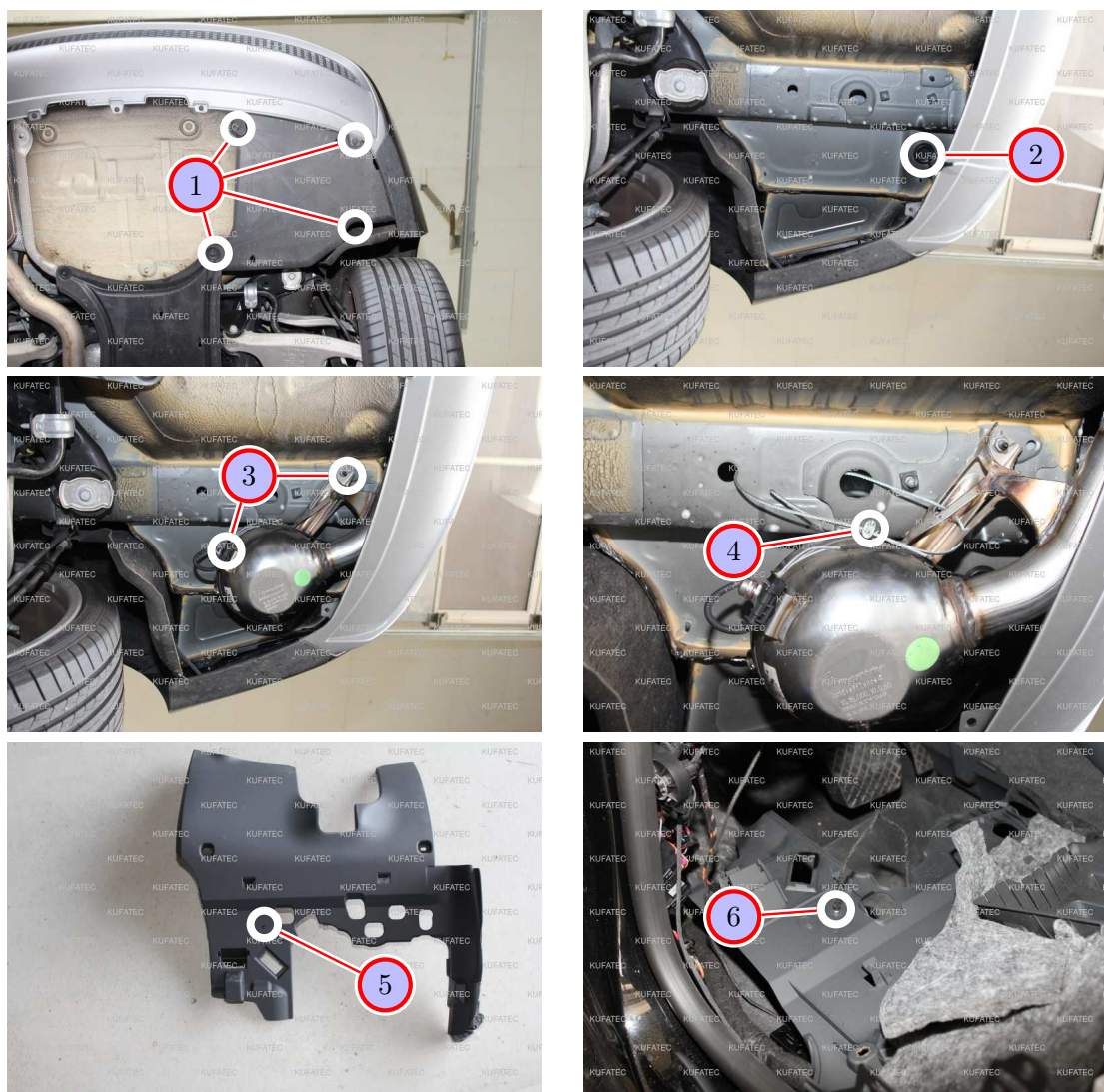
Figure 9: Installation sound generator and pushbutton
