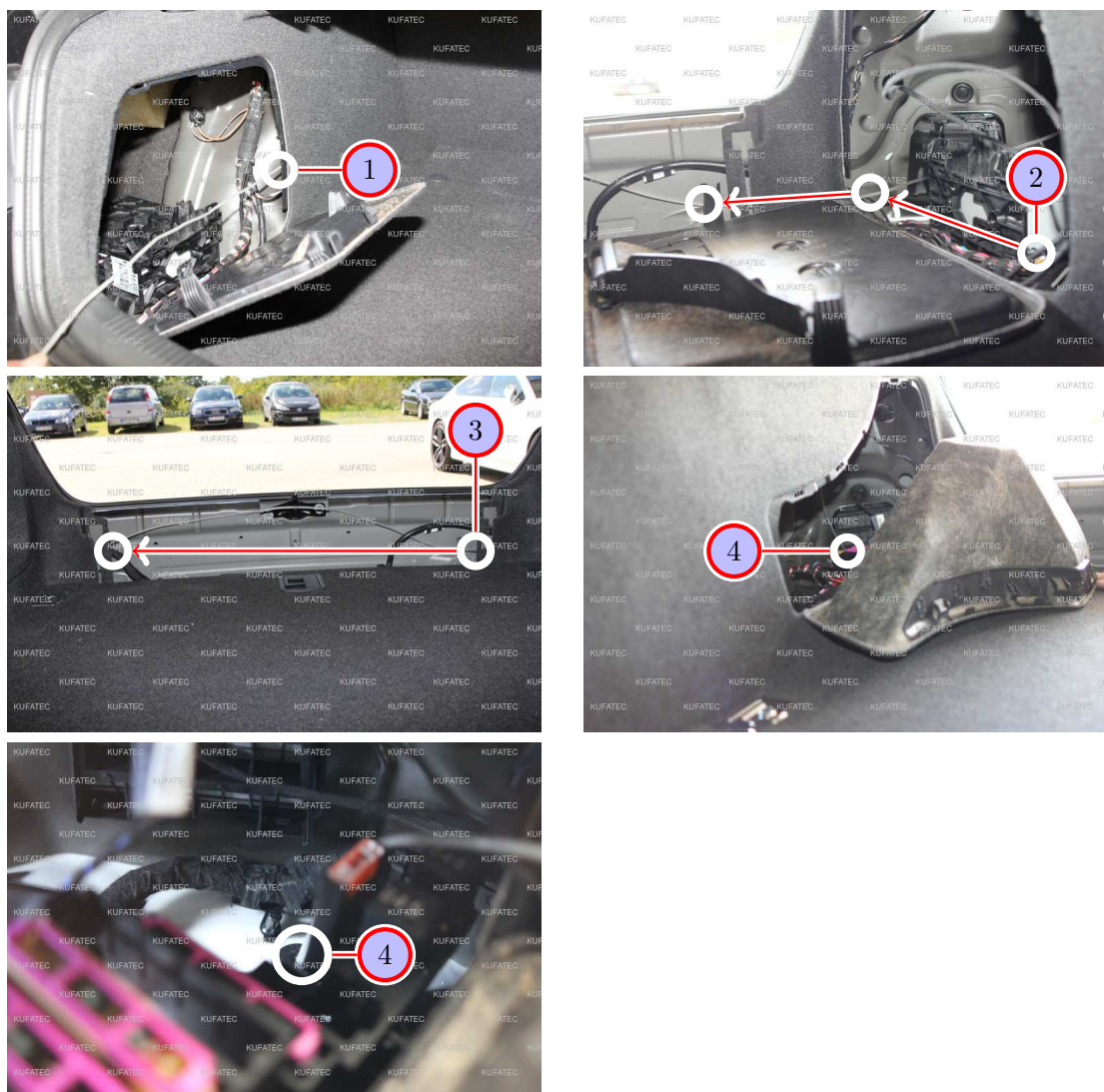
Figure 8: Cable routing trunk
