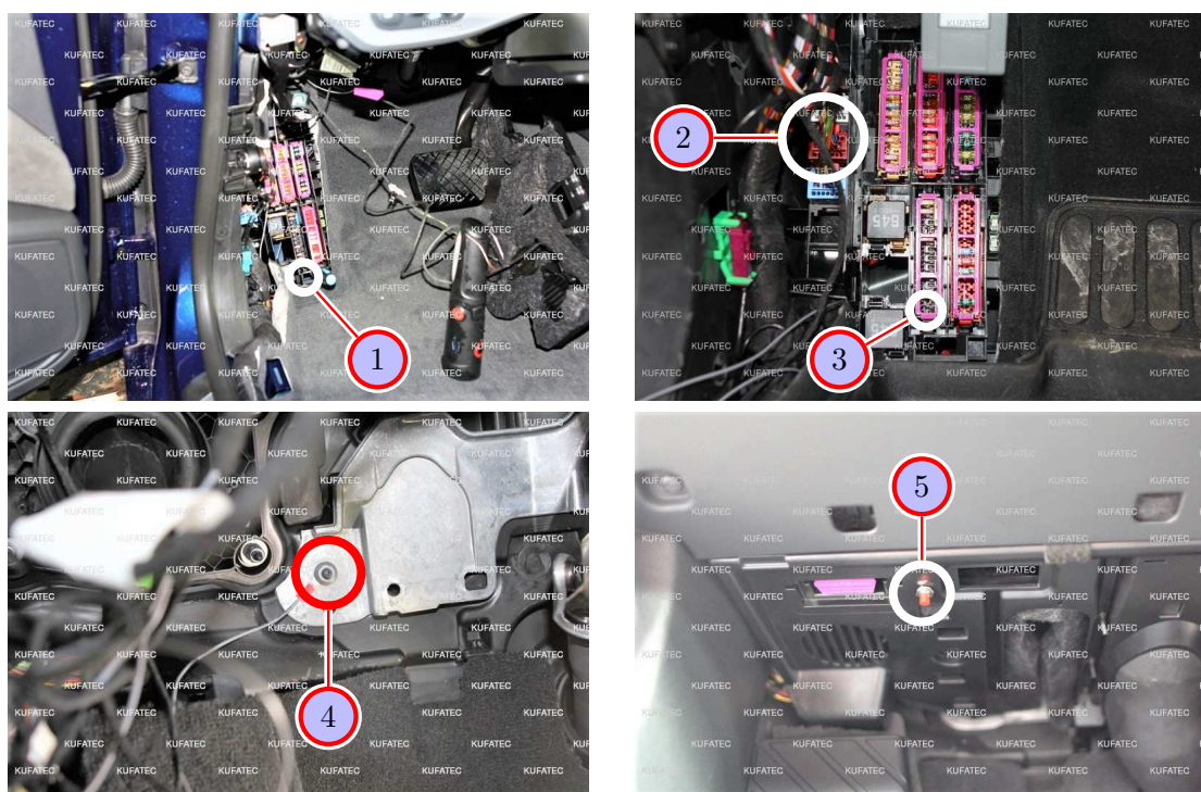
Figure 7: Connection Can high + low / Ground / Pushbutton
